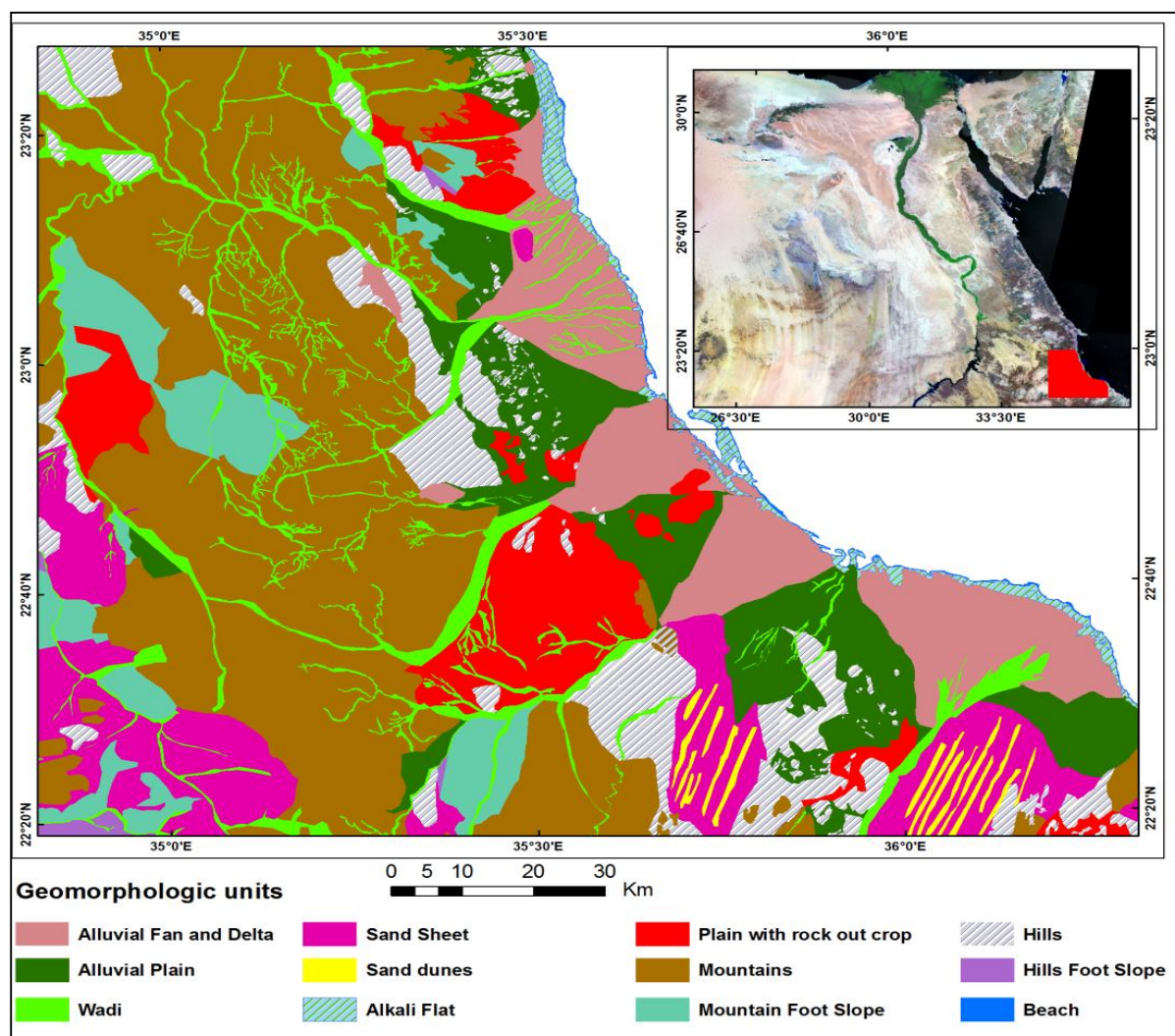
Fig. 4: Geomorphic map of the Hala'ib and Shalateen area.
